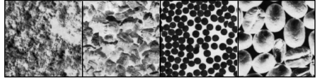
Figure 2. Samples for classes D002, D005, D067 and D074 (left to right).
