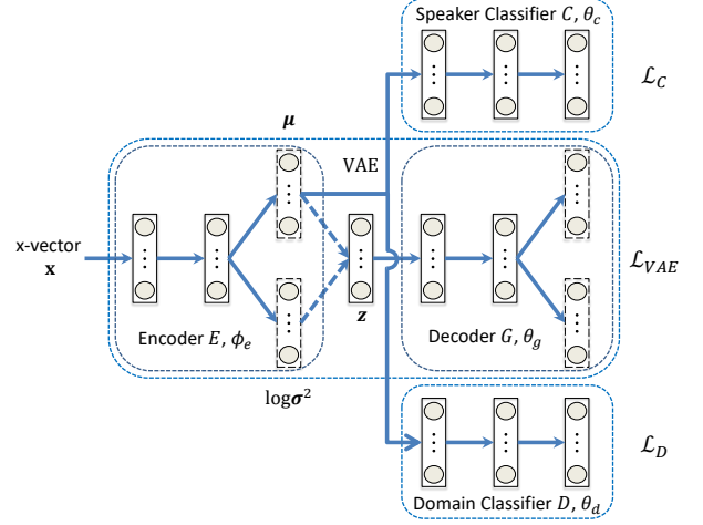
Figure 1: Schematic of VDANN. The solid and dashed arrows represent network connections and stochastic sampling, respectively.
