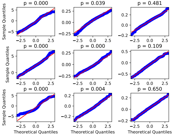
Figure 2: Quantile-quantile (Q-Q) plots of the 11-th (the 1st row), 111-th (the 2nd row), and 211-th (the 3rd row) components of x-vectors (the 1st column), DANN-transformed x-vectors (the 2nd column), and VDANN-transformed x-vectors (the 3rd column). The vertical and horizontal axes correspond to the samples under test and the samples drawn from a standard normal distribution, respectively. The red line represents the situation of perfectly Gaussian. The p-values above the graphs were obtained from Shapiro–Wilk tests in which p > 0.05 means failing to reject the null hypothesis that the test samples come from a Gaussian distribution.
